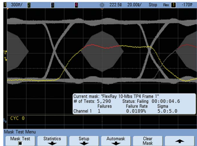
Figure 9. A “stop-on-error” TP4-10Mbps mask test.
